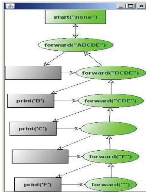
Figure 4. An RGraph for Forward Printing of list "ABCDE" with 30% of labels missing
