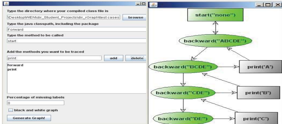
Figure 1. RGraph Software Tool – User Interface Panel
